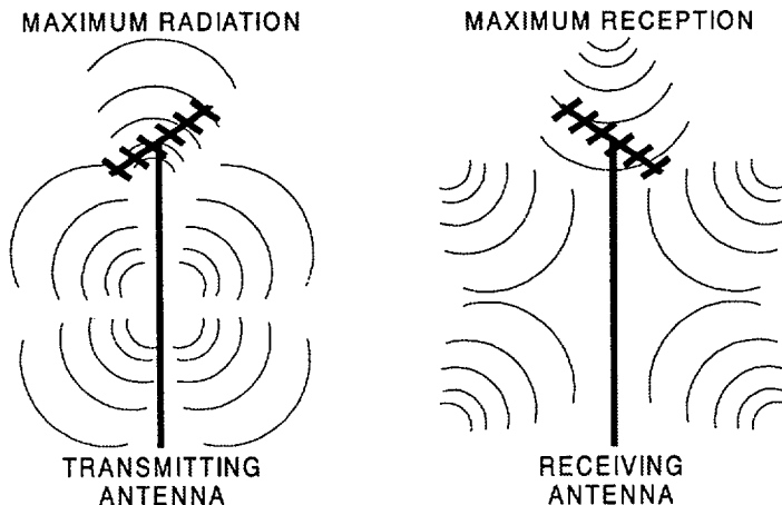
Figure 2-6. Reciprocity.
