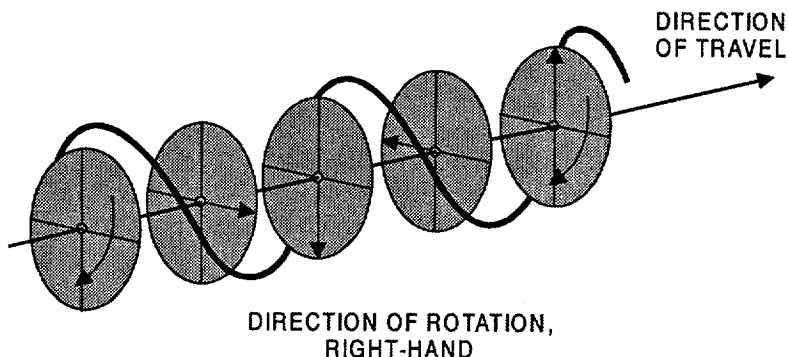
Figure 2-5. Circular Polarization.
