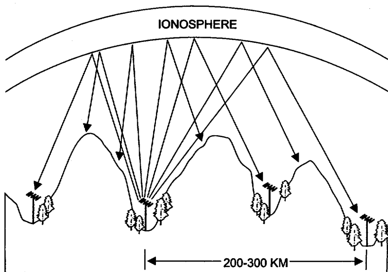
Figure 4-33. NVIS Propagation.
