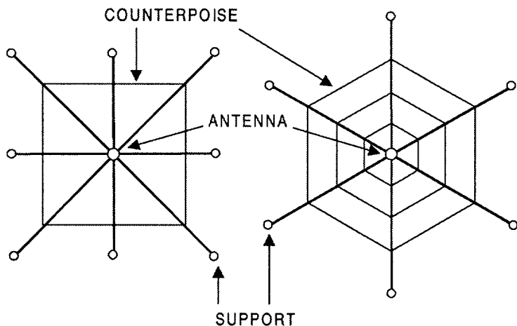
Figure 2-10. Wire Counterpoise.
