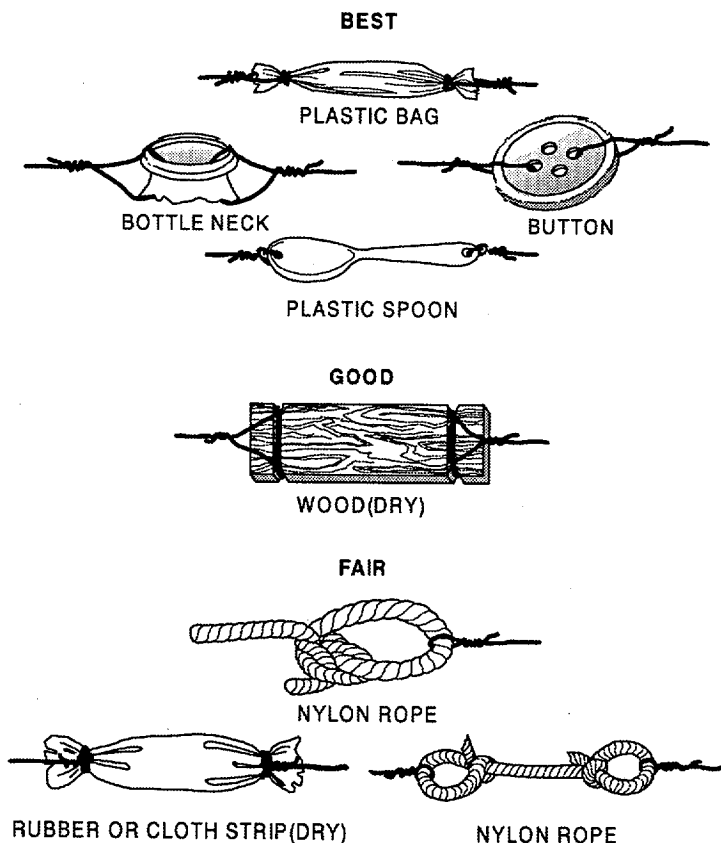
Figure 6-2. Improvised Insulators.
