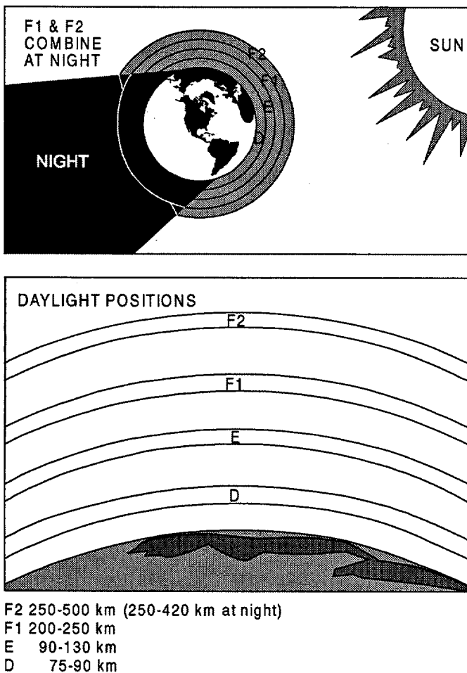
Figure 1-5. Ionospheric Structure.
